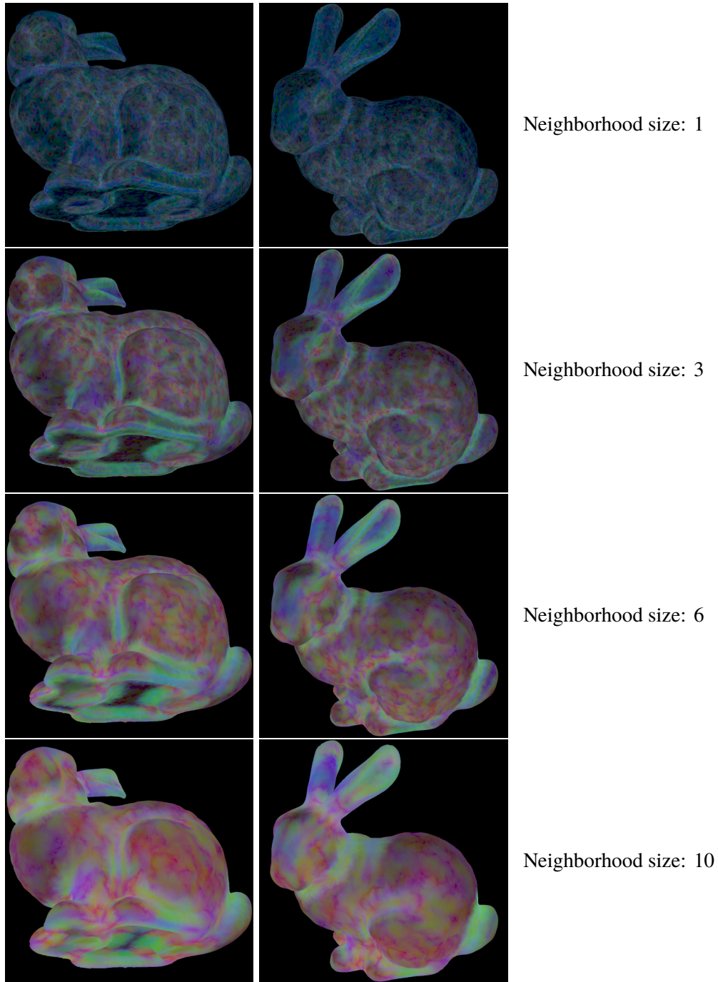
Figure 1: Bunny model color coded according to the magnitude of the three smallest eigenvalues on local neighborhoods. The four rows of the table correspond to evaluating C over neighborhoods of radius 1, 3, 6, and 10 edges. The color coding is such that black regions correspond to 3 small eigenvalues, blue to 2 small eigenvalues, green to 1 small eigenvalue, and red to no small eigenvalues.
